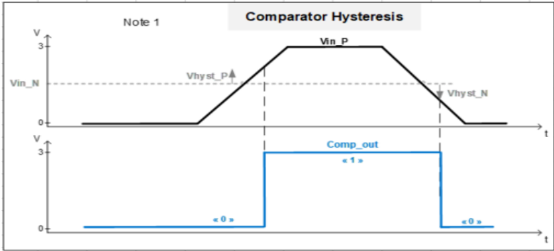
Fig 21. Comparator Hysteresis
