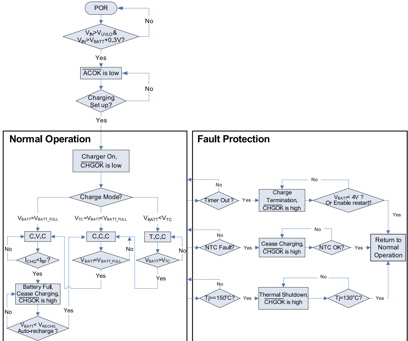
Figure 4: Operation Flow Chart
