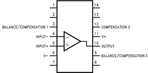
Dual-In-Line Package
