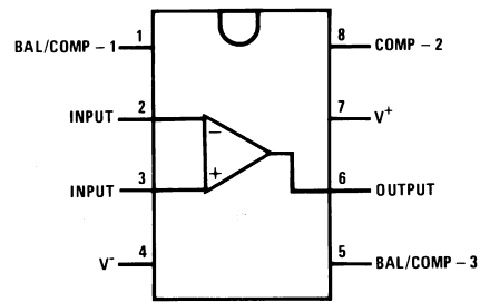
Dual-In-Line Package
