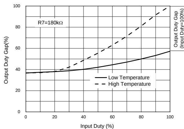
Output PWM Duty vs. Input PWM Duty with R7 (180k \Omega )
