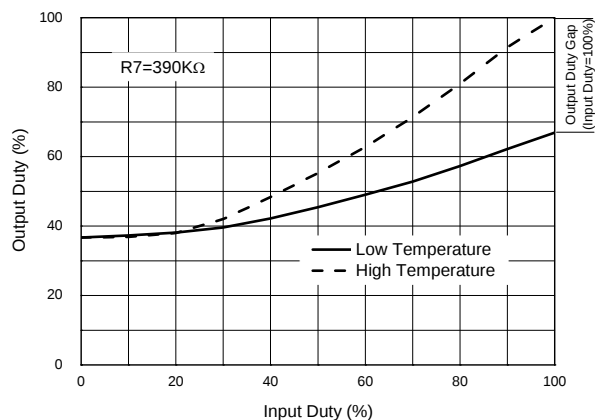
Output PWM Duty vs. Input PWM Duty with R7 (390k \Omega )
