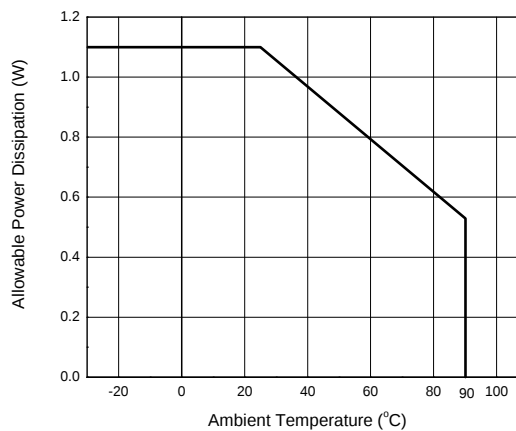
Allowable Power Dissipation vs. Allowable Temperature (Note 6)
