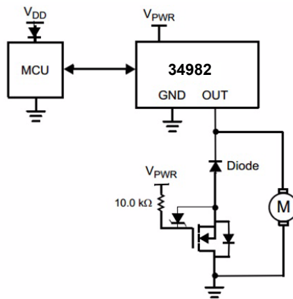
Figure 10. Reverse Voltage Protection
