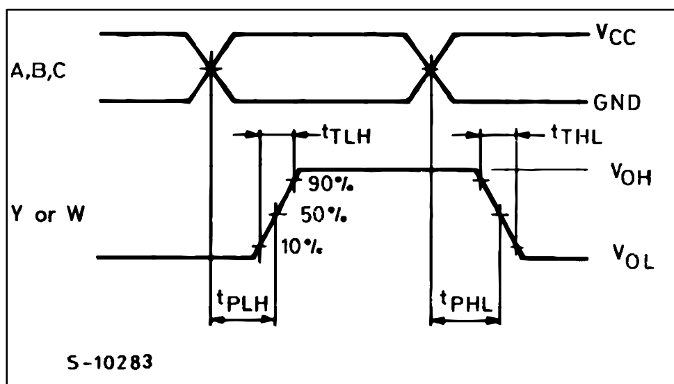
Figure 6: Waveform 2: propagation delay times ( f = 1\text{ MHz} ; 50% duty cycle)
