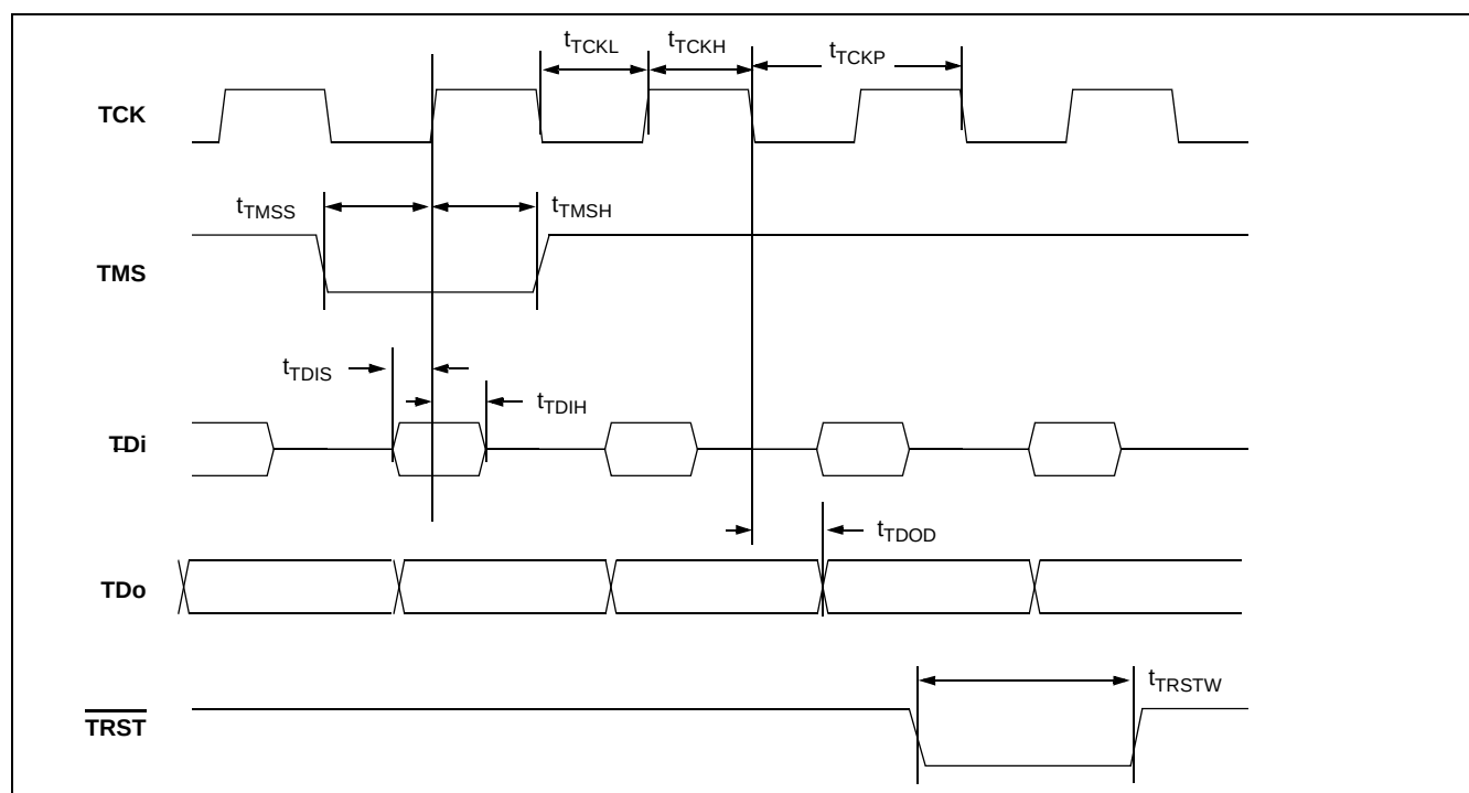
Figure 27 - JTAG Test Port Timing Diagram
