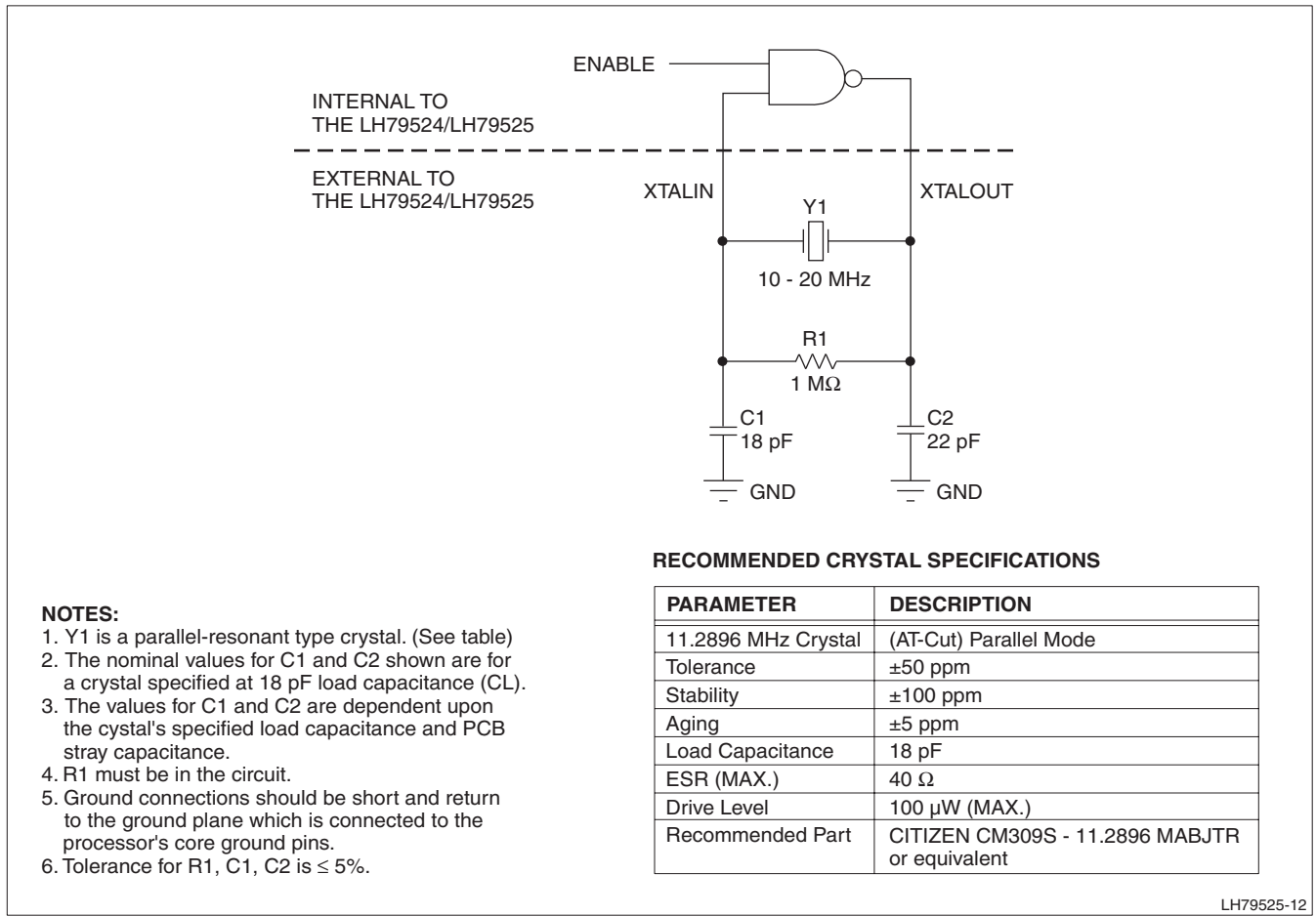
Figure 38. Suggested External Components, 10 - 20 MHz Oscillator
