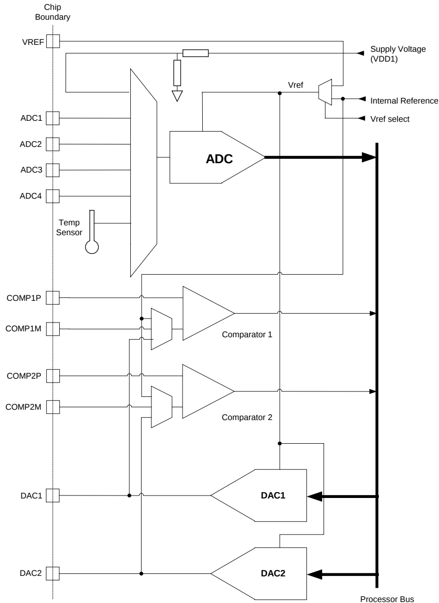
Figure 43: Analogue Peripherals
