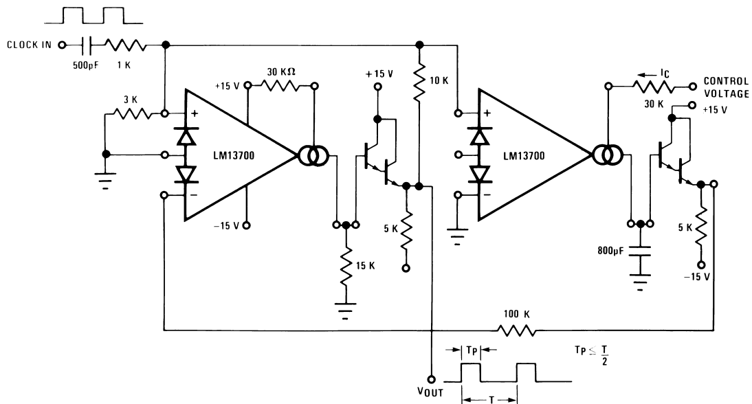
Figure 47. Pulse Width Modulator
