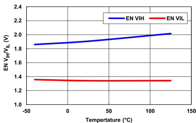
Figure 11. EN V_{IL} and V_{IH} vs Temperature
