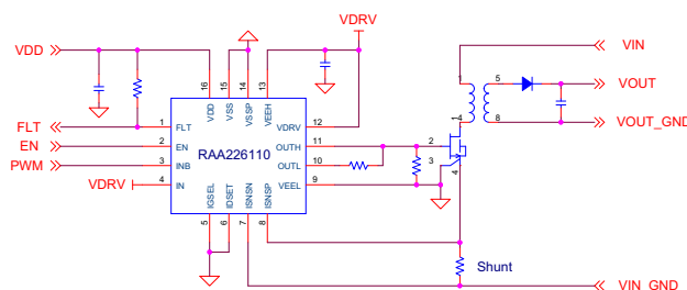
Figure 2. Typical Inverting Input
