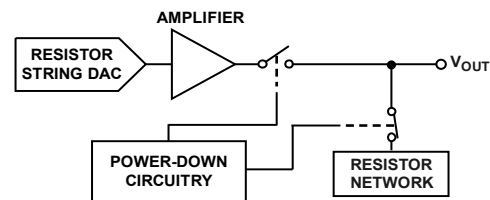
Figure 29. Output Stage During Power-Down
