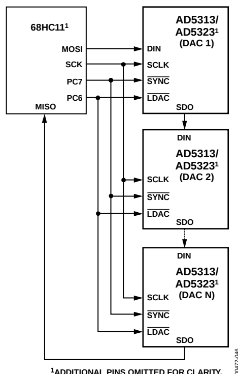
Figure 41. Daisy-Chain Mode
