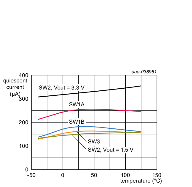
Figure 18. Quiescent current Buck regulators in APS mode
