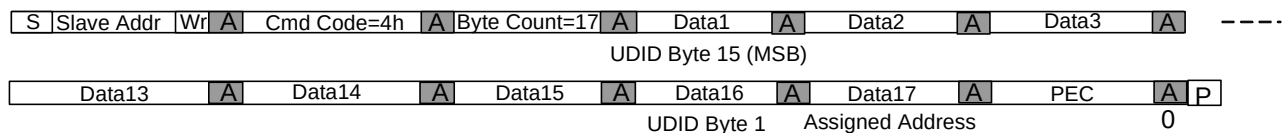
Figure 7-18. Assign SMBus Address ARP Command Format
