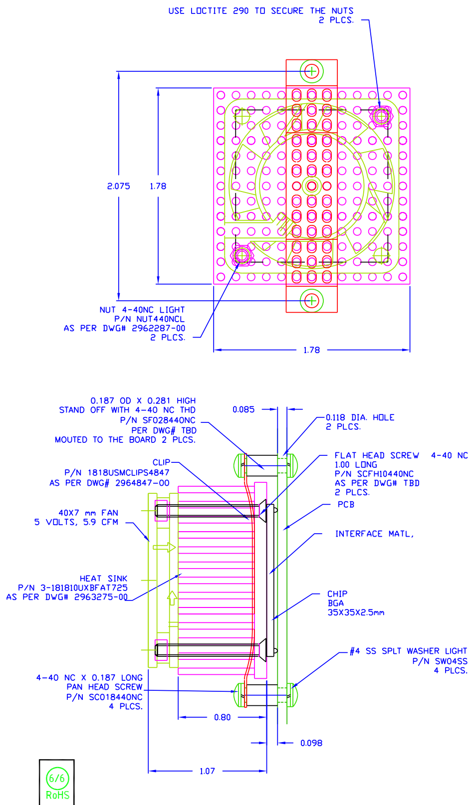
Figure 19-1. Extended Temperature Thermal Solution
