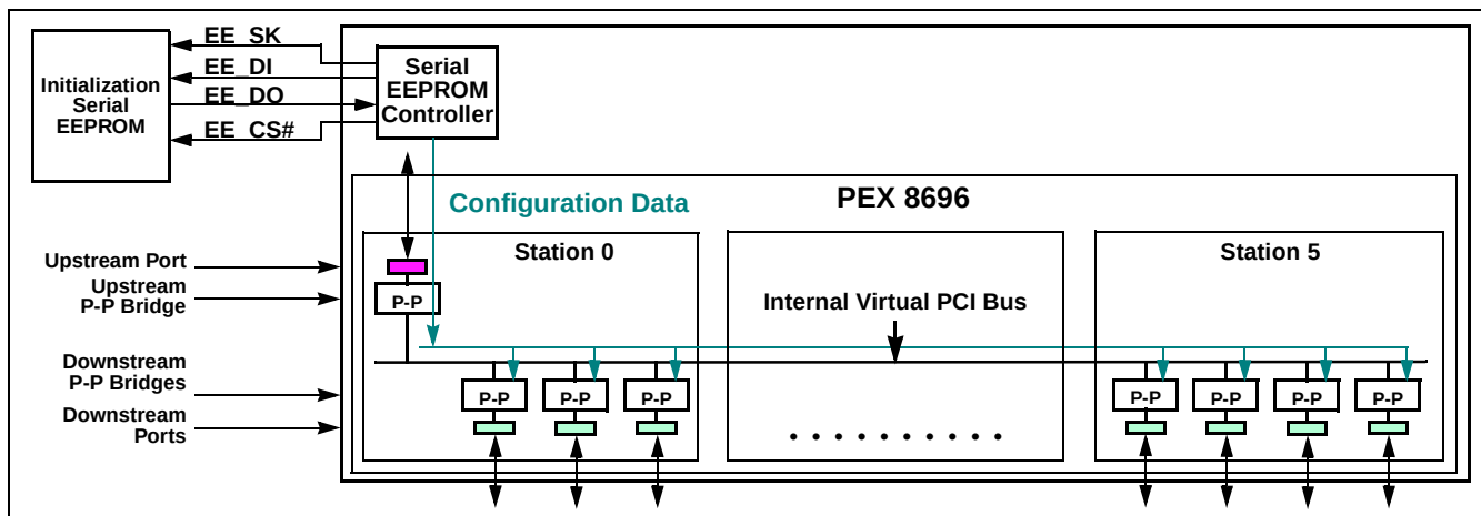
Figure 6-1. Serial EEPROM Connections
