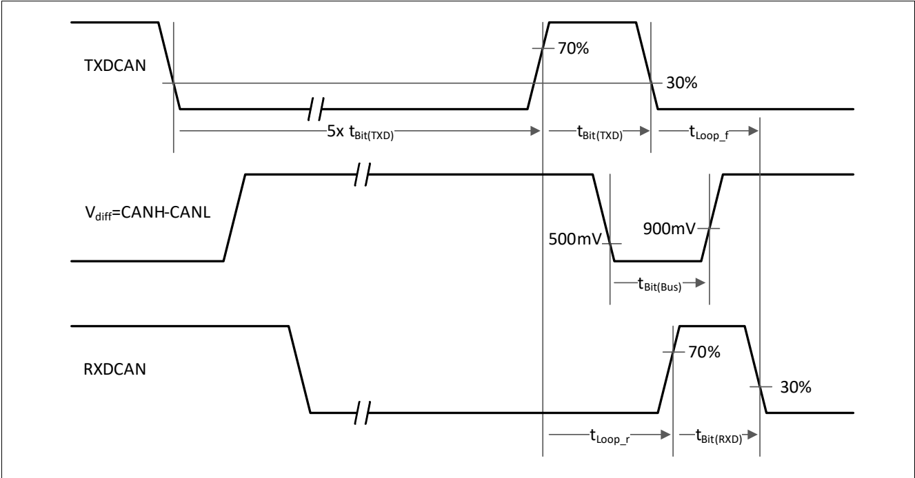
Figure 29 From ISO 1198-2: tloop, tbit(TXD), tbit(Bus), tbit(RXD) definitions
