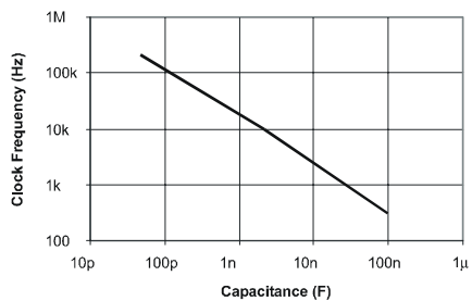
Clock Frequency v Capacitance
