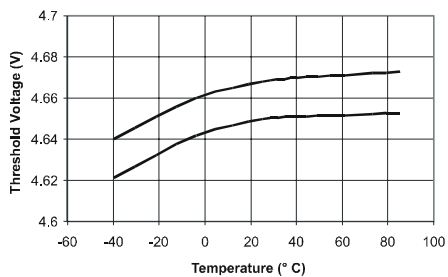
Threshold Voltage v Temperature
