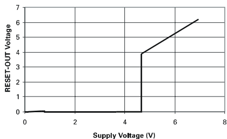
RESET-OUT Voltage v Supply Voltage
