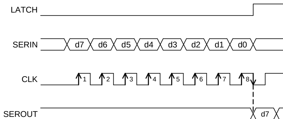
Figure 6. SEROUT Output Signal
