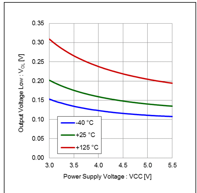
Figure 15. Output Voltage Low vs Power Supply Voltage (@I SO (Note 3)=4 mA)
