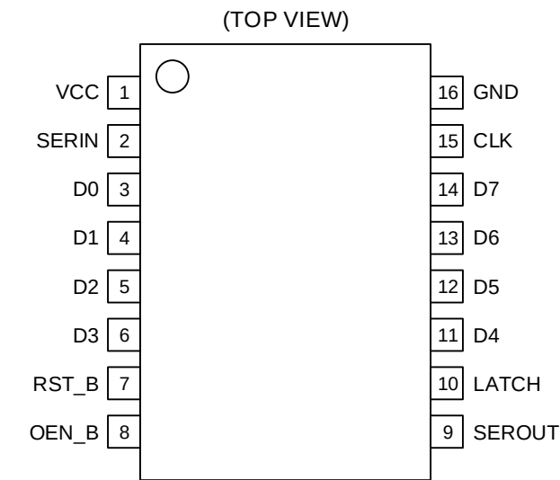
Figure 2. Pin Configuration
