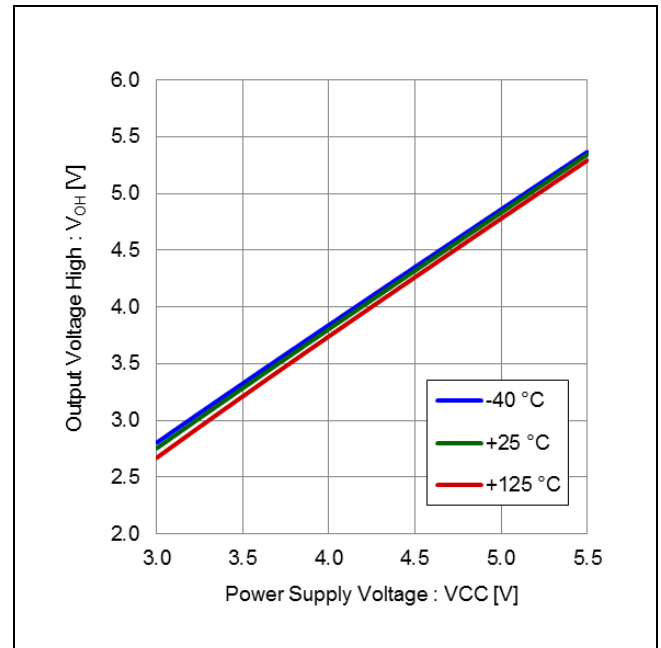
Figure 13. Output Voltage High vs Power Supply Voltage (@I SO (Note 3)=-4 mA)
