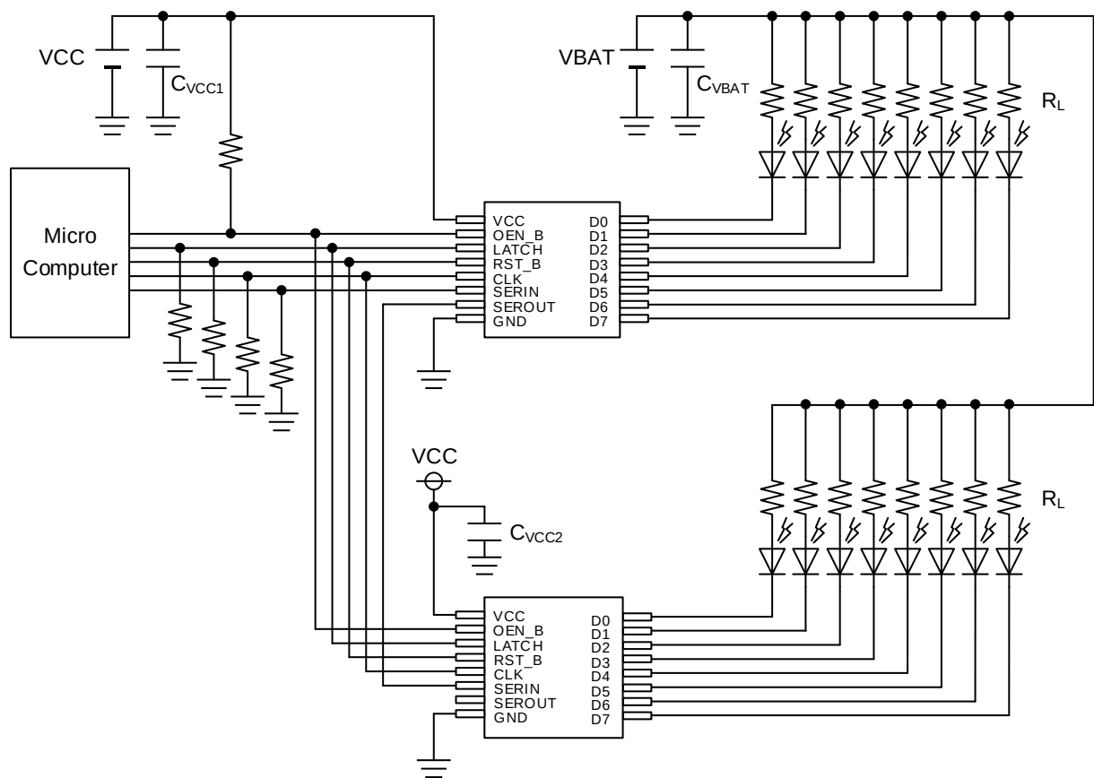
Figure 19. Application Example
