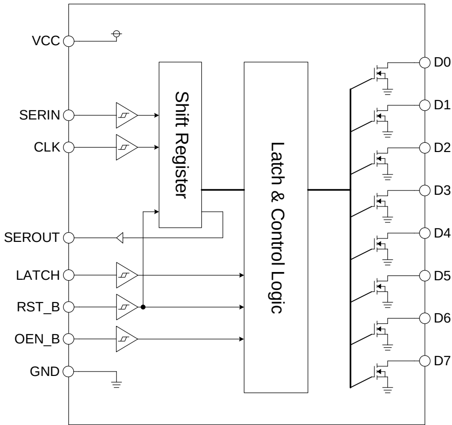
Figure 3. Block Diagram
