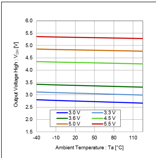
Figure 14. Output Voltage High vs Ambient Temperature (@I SO (Note 3)=-4 mA)
