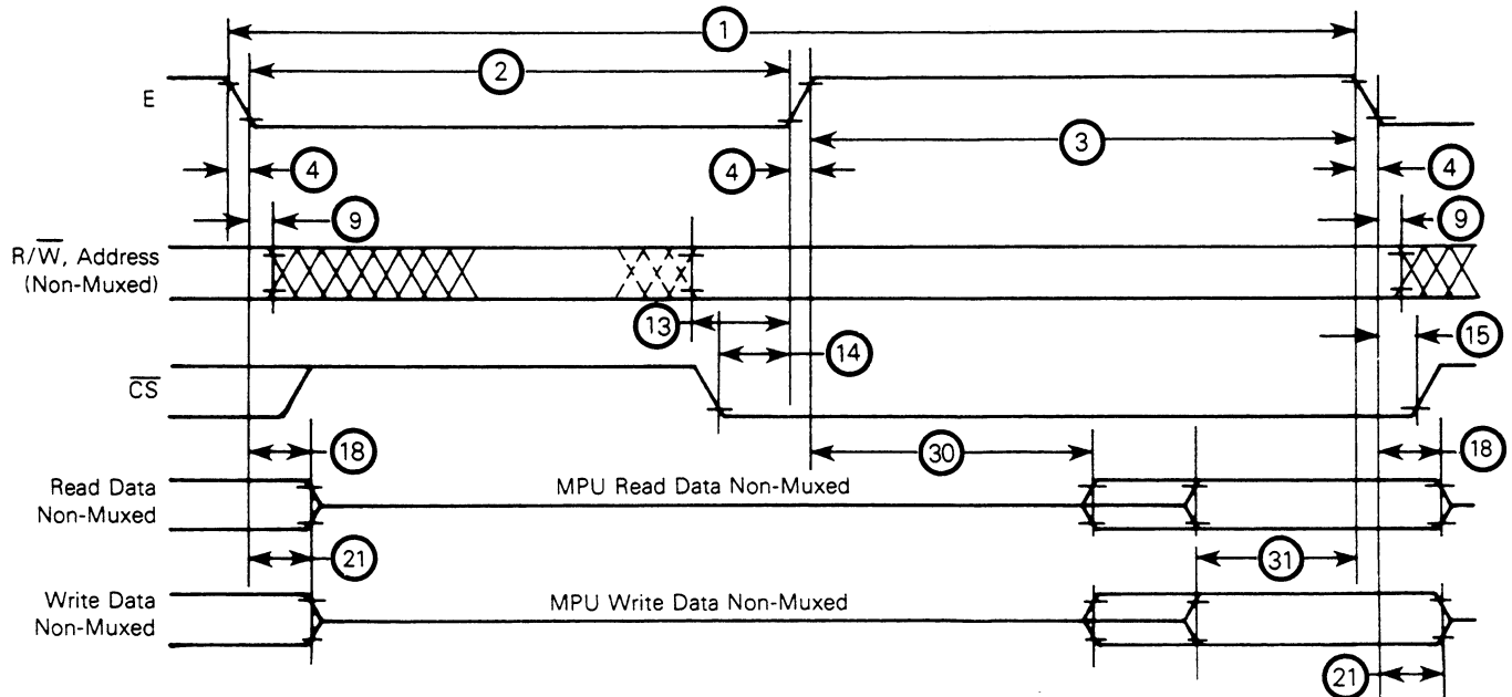
FIGURE 1 — BUS TIMING
