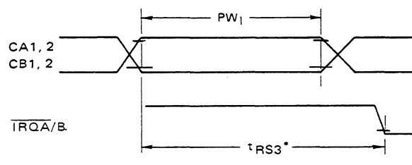
FIGURE 13 — INTERRUPT PULSE WIDTH AND \overline{\text{IRQ}} RESPONSE
