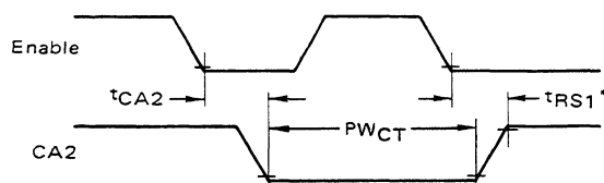
FIGURE 7 — CA2 DELAY TIME (Read Mode; CRA-5=CA3=1, CRA-4=0)
