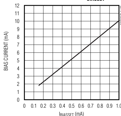
BIAS CURRENT vs. I_{BIASSET}
