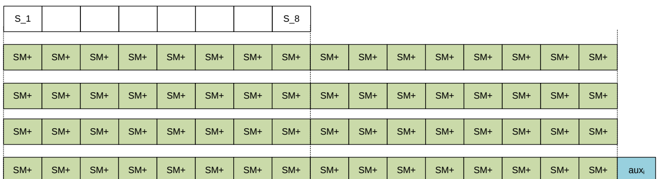
Figure 25: Sequencer Setup for Highest Update Rate on Bridge Sensor
