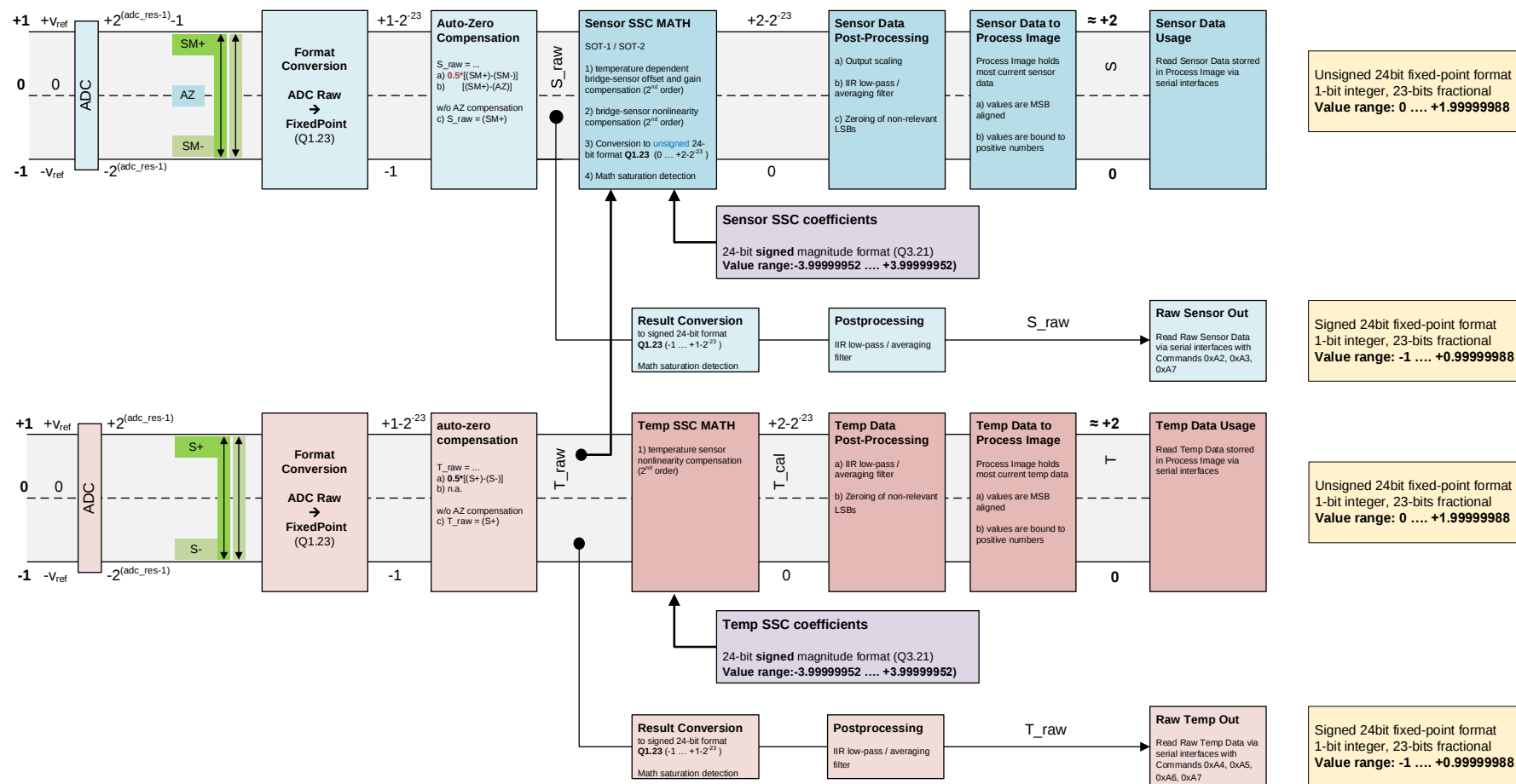
Figure 29: SSC Signal Data Path
