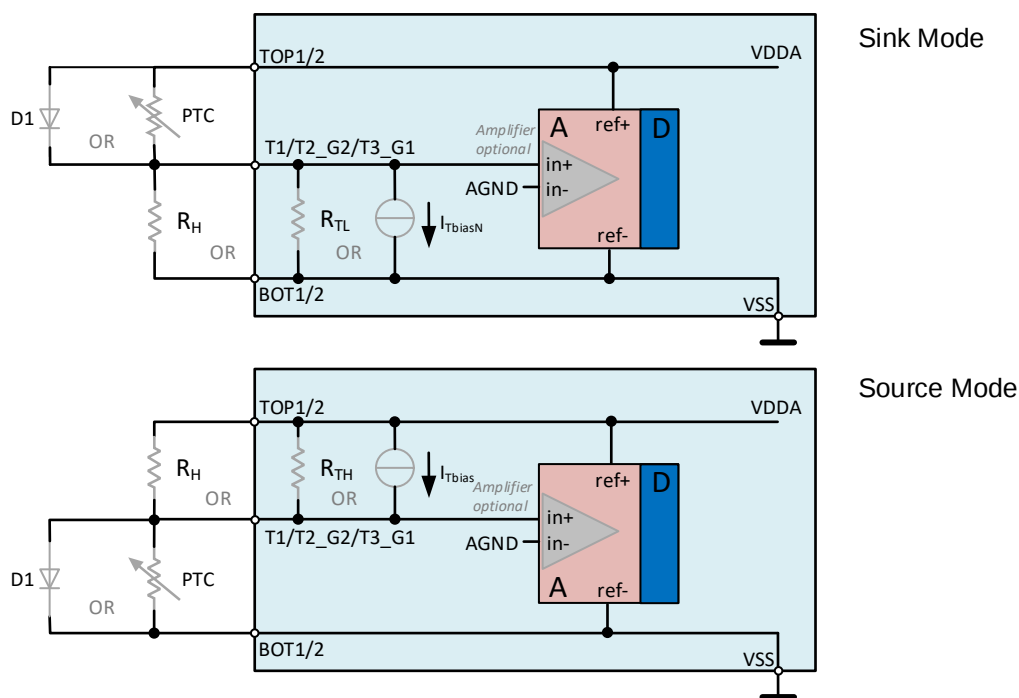
Figure 11: PTC, Diode Sensor Bias Configurations
