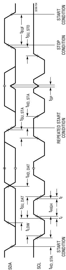
Figure 4. Timing Parameters
