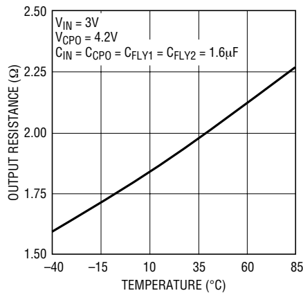
1.5x Mode Charge Pump Open-Loop Output Resistance vs Temperature ( 1.5V_{IN} - V_{CP0} )/ I_{CP0}
