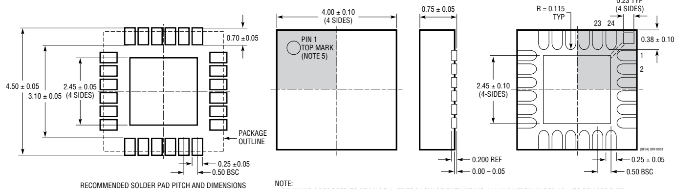
UF Package 24-Lead Plastic QFN (4mm × 4mm) (Reference LTC DWG # 05-08-1692)
