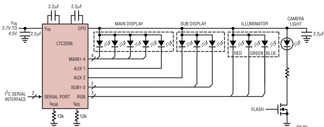
4-Display Controller
