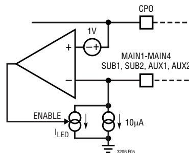
Figure 5. Internal MAIN, SUB and AUX LED Disable Circuit
