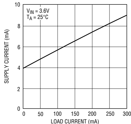
1.5x Mode Supply Current vs ICP0 ( I_{IN} - 1.5I_{CP0} )
