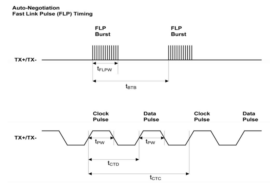
Figure 14. Auto-Negotiation Fast Link Pulse (FLP) Timing
