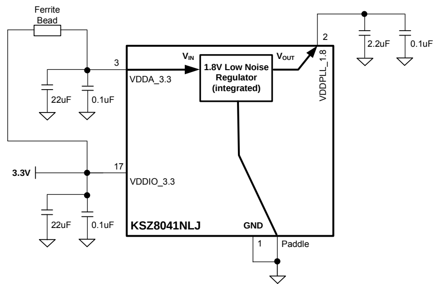
Figure 6. KSZ8041NLJ Power and Ground Connections
