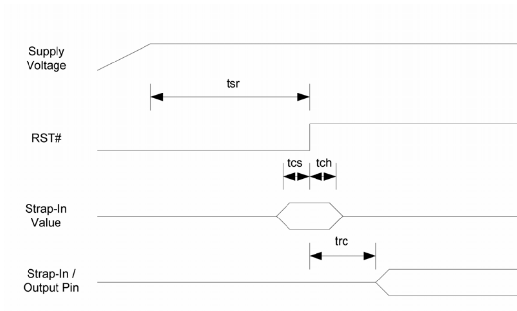
Figure 16. Reset Timing
