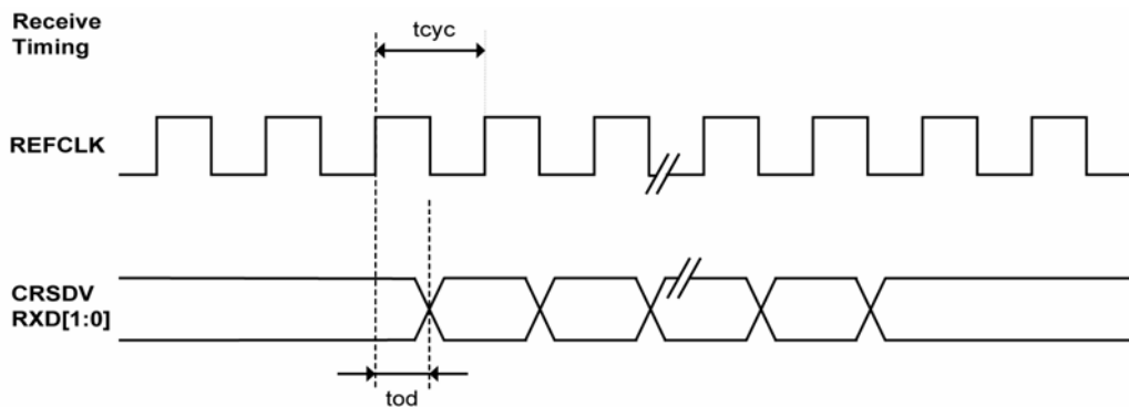
Figure 13. RMII Timing – Data Input to RMII
