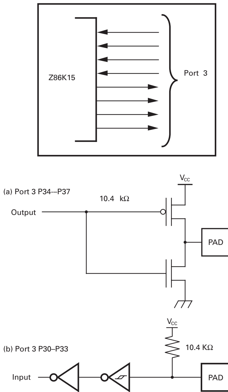
FIGURE 8. PORT 3 CONFIGURATION
