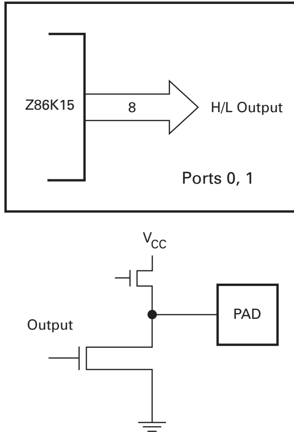
FIGURE 6. PORTS 0 AND 1 CONFIGURATION
