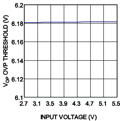
V_{OVP} vs. V_{IN}
