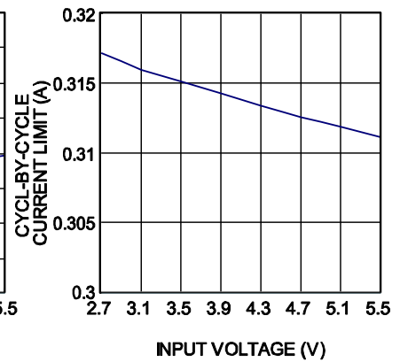
Current Limit vs. V_{IN}
