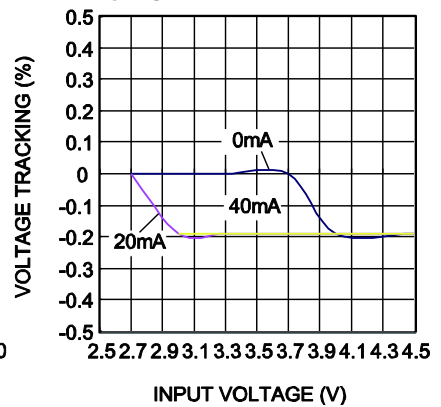
Voltage Tracking @ Symmetric Load
