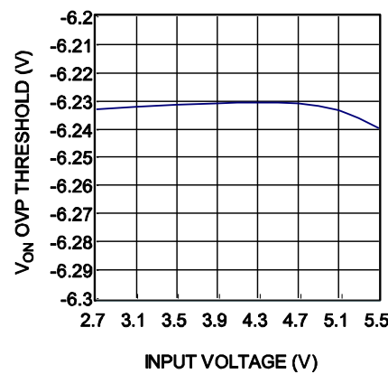
V_{OVN} vs. V_{IN}
