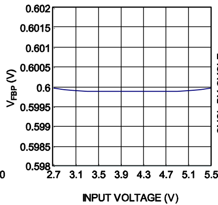
V_{FBP} vs. V_{IN}
