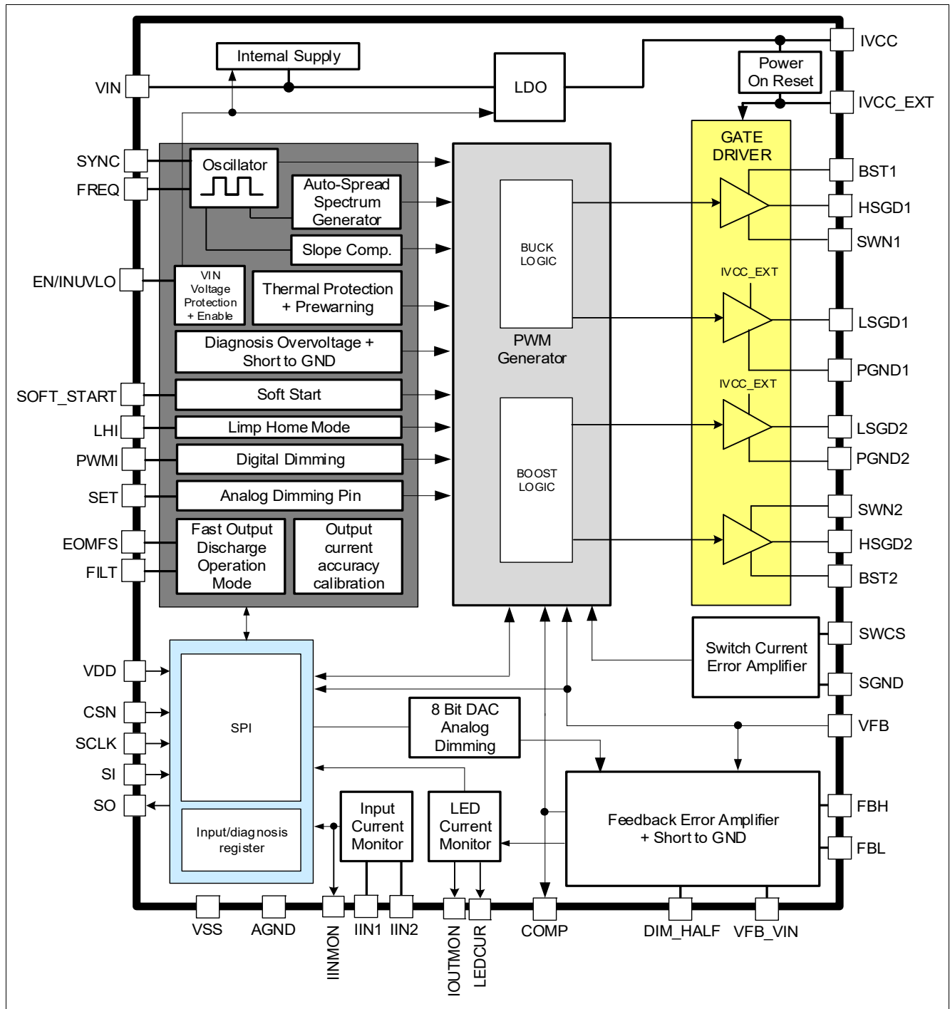
Figure 2 Block Diagram - TLD5542-1
