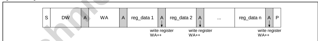
Figure 23. Page Write
