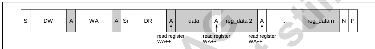
Figure 25. Sequential Read
