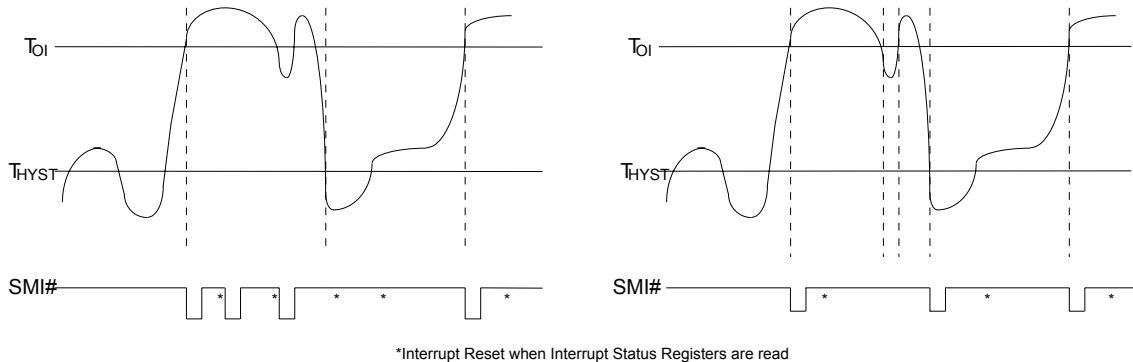
Figure 16-1. Comparator Interrupt Mode
