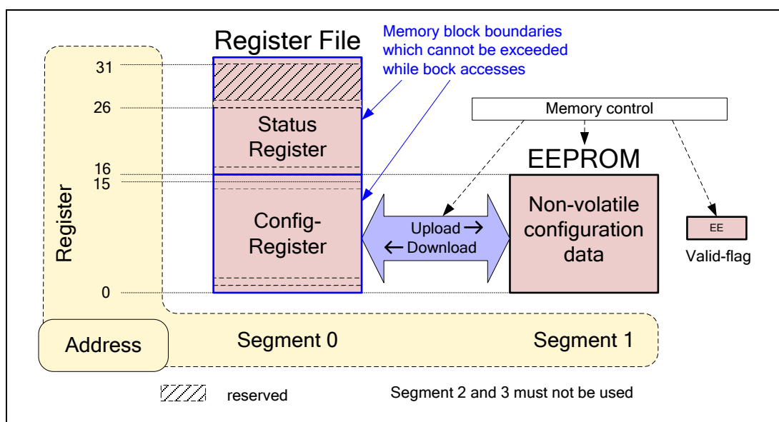
Figure 3.9 Memory Unit
