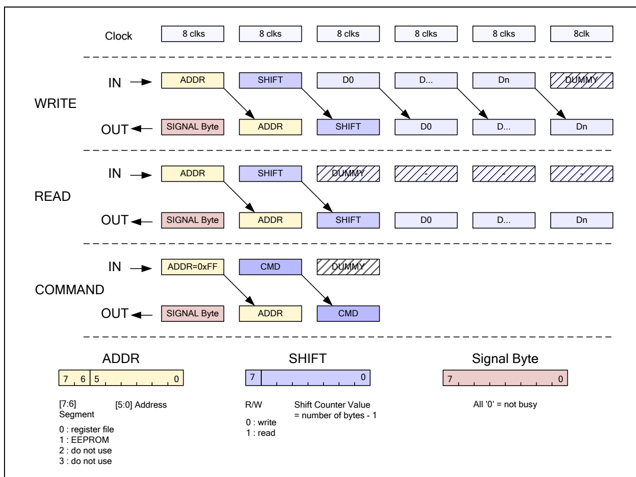
Figure 3.11 Structure of SPI accesses
