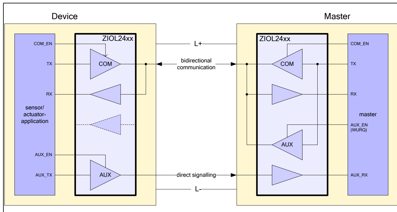
Figure 3.5 ZIOL24xx in Device and Master Mode Application
