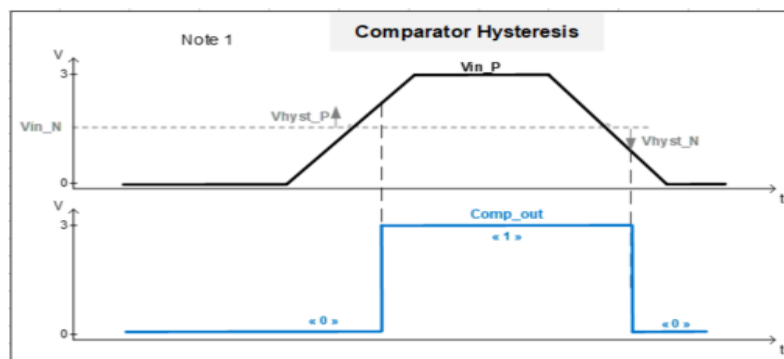
Fig 22. Comparator Hysteresis
