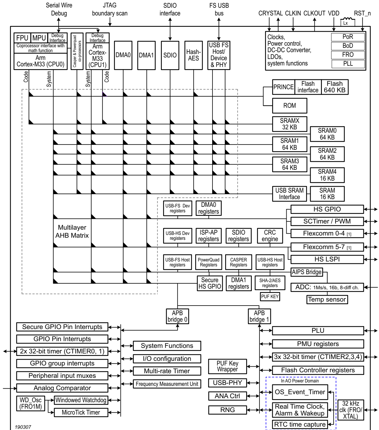
Fig 3. LPC55S6x Block diagram
