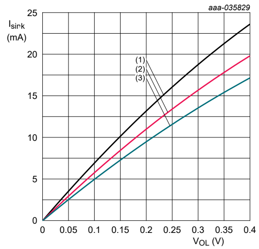
b. V_{\text{CC}} = 1.8 \text{ V}
