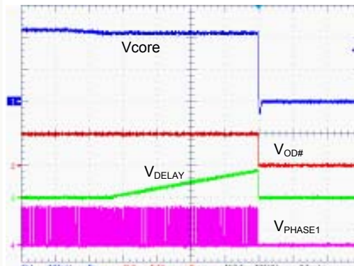
Figure 11. Over-Current Latch-off Waveforms
