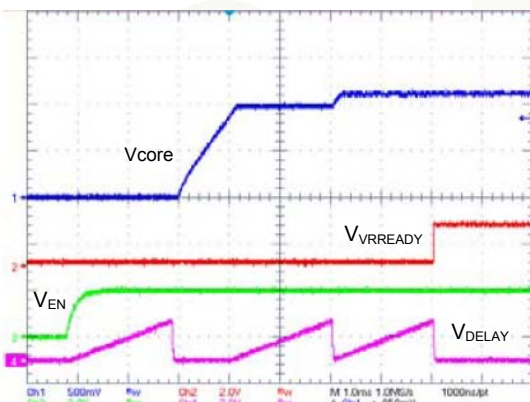
Figure 10. Start-up Waveforms
