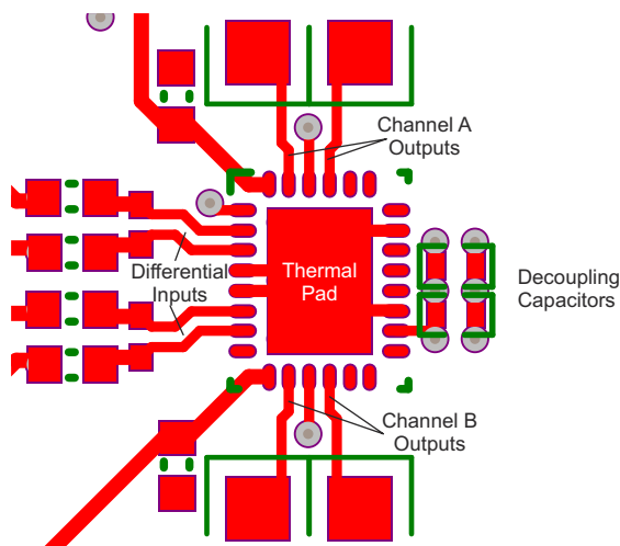
Figure 10-1. Example Layout
