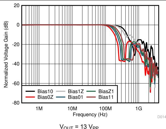
Figure 6-14. Normalized Large-Signal Frequency Response
