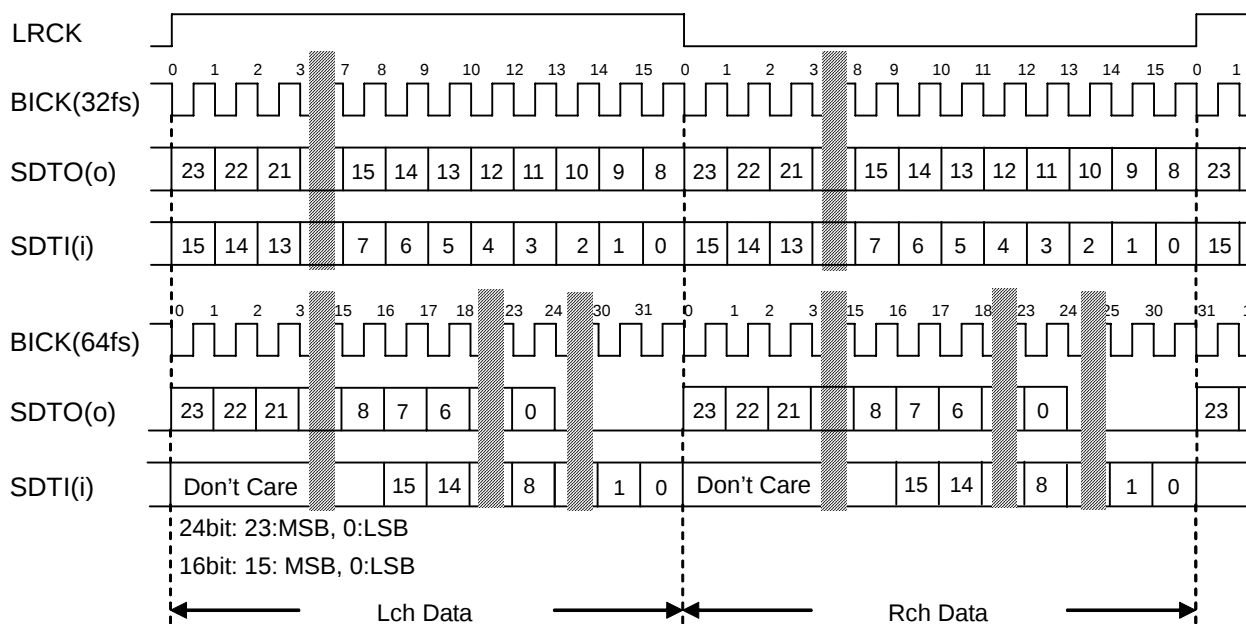
Figure 24. Mode 1 Timing
