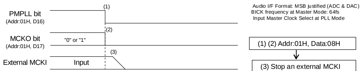
Figure 76. Clock Stopping Sequence (1)
