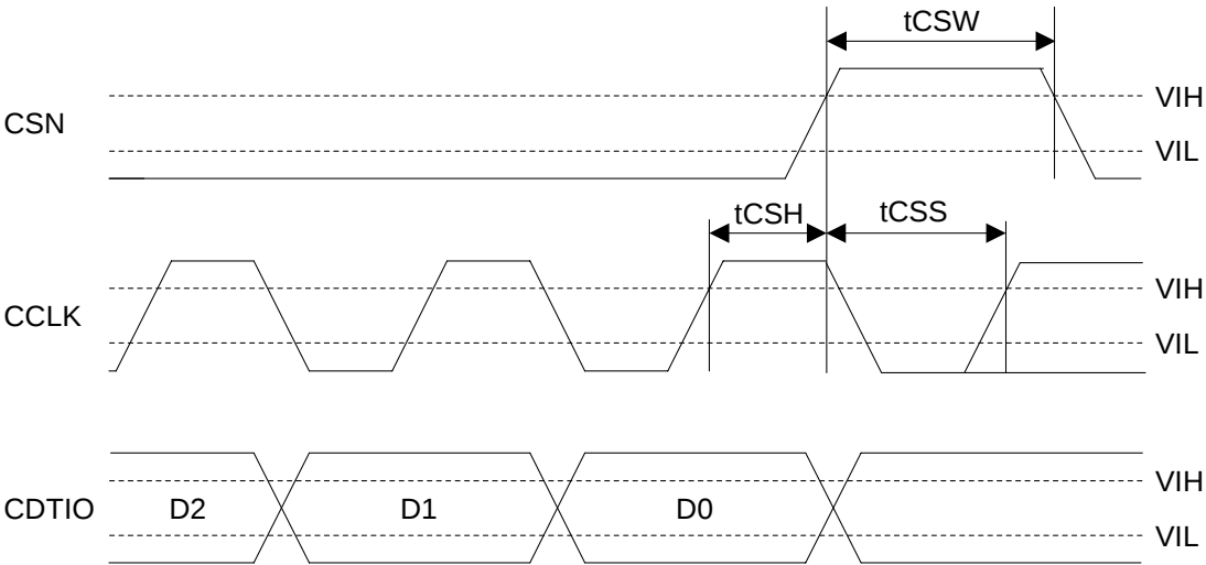
Figure 10. WRITE Data Input Timing
