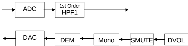
Figure 35. The Path in Recording Mode 2 & Playback Mode 2
