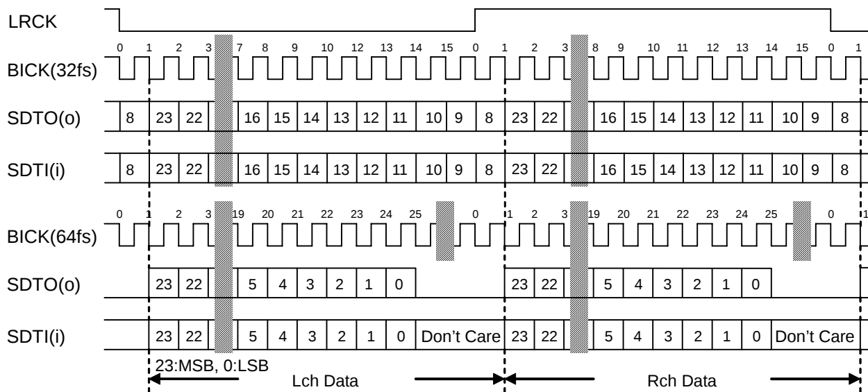
Figure 26. Mode 3 Timing
