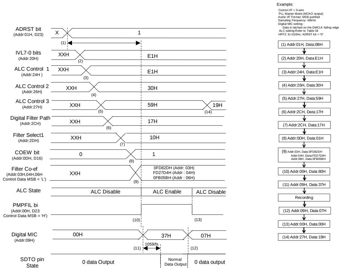
Figure 71. Digital MIC Input Recording Sequence
