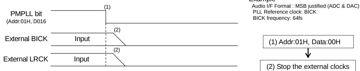
Figure 77. Clock Stopping Sequence (2)
