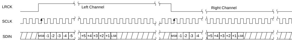
Figure 31. Left-Justified Serial Audio Formats
