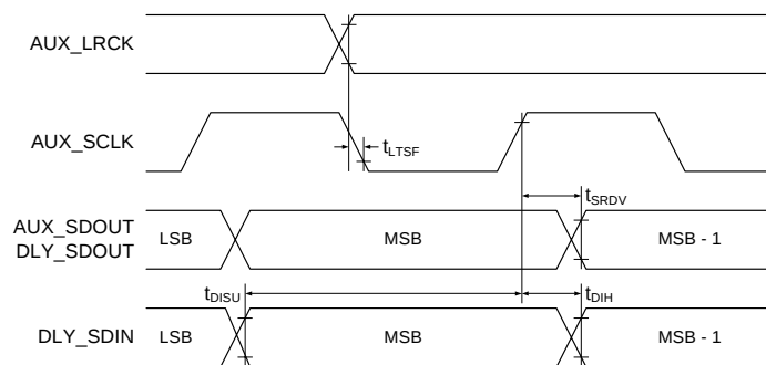
Figure 8. AUX Serial Port Interface Master Mode Timing
