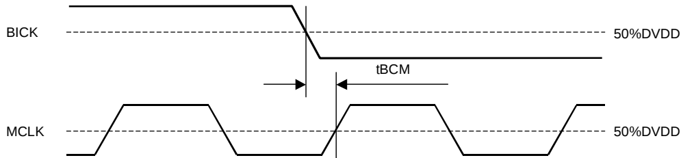
Figure 12. I 2 S Compatible
