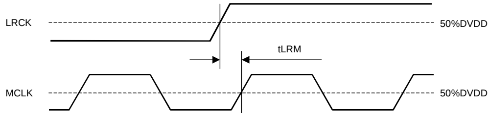
Figure 11. 16/20/24bit LSB Justified, 24bit MSB Justified
