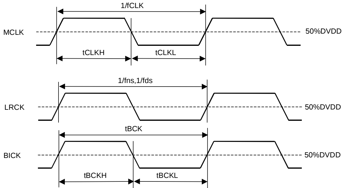
Clock Timing
