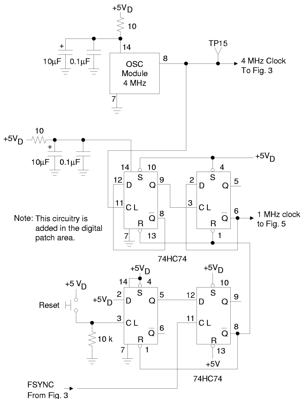
Figure 2. Clock Oscillator/Divider
