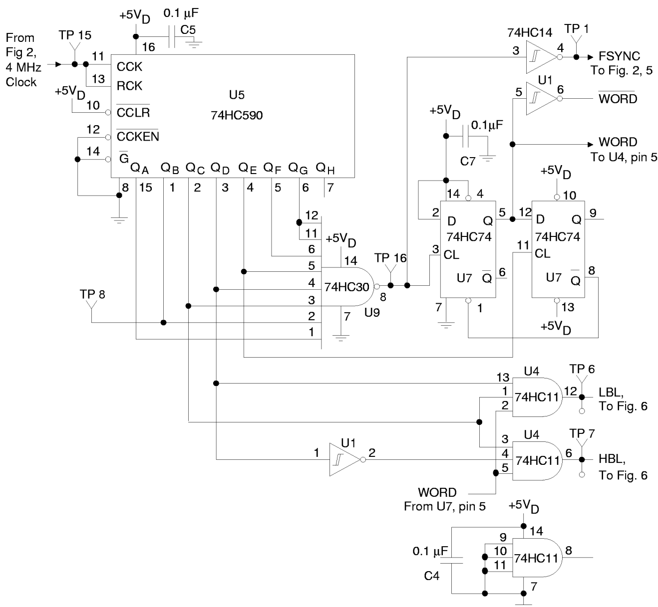
Figure 3. Timing Generator
