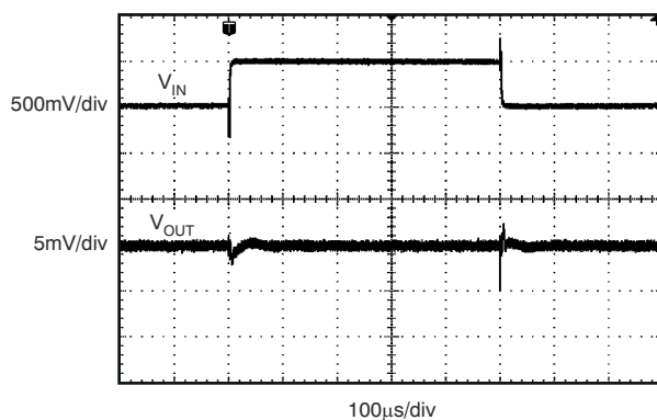
Figure 7-22. Line Transient
