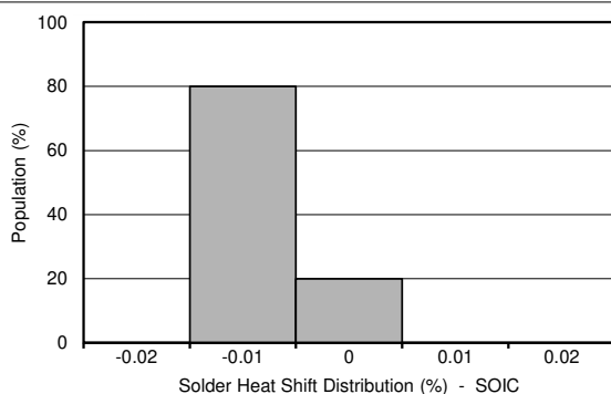
Figure 8-2. Solder Heat Shift Distribution (%), SOIC Package
