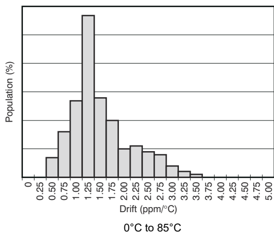
Figure 7-1. Temperature Drift
