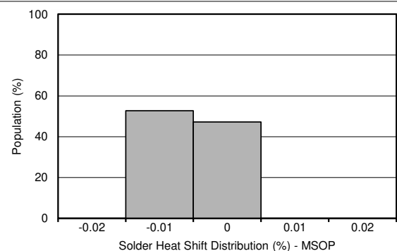
Figure 8-3. Solder Heat Shift Distribution (%), VSSOP Package
