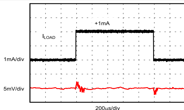
Figure 7-19. Load Transient
