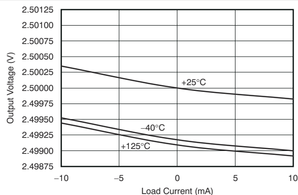
Figure 7-7. REF5025 Output Voltage vs Load Current
