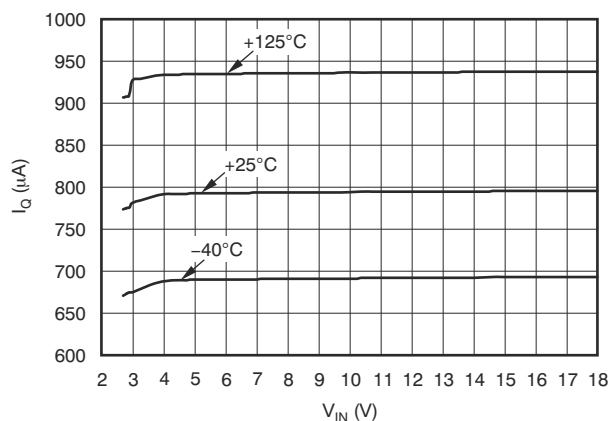
Figure 7-10. Quiescent Current vs Input Voltage
