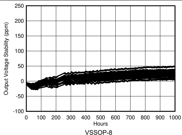
Figure 7-23. REF50xx Long-Term Stability (First 1000 Hours)
