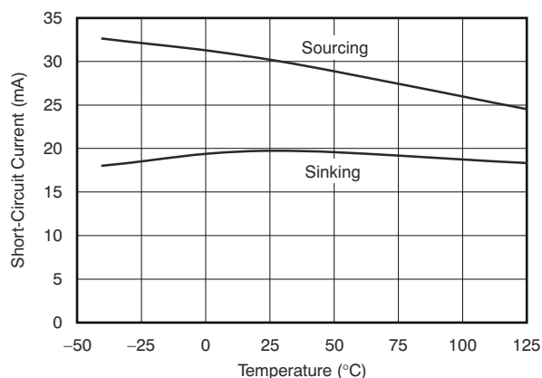
Figure 7-12. Short Circuit Current vs Temperature
