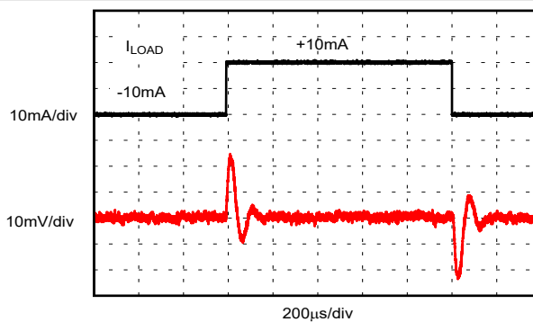
Figure 7-20. Load Transient
