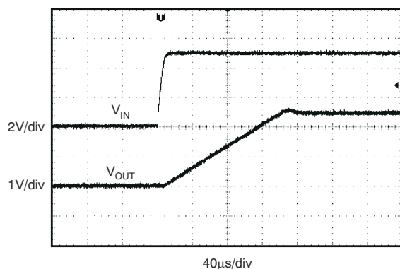
Figure 7-15. Start-Up
