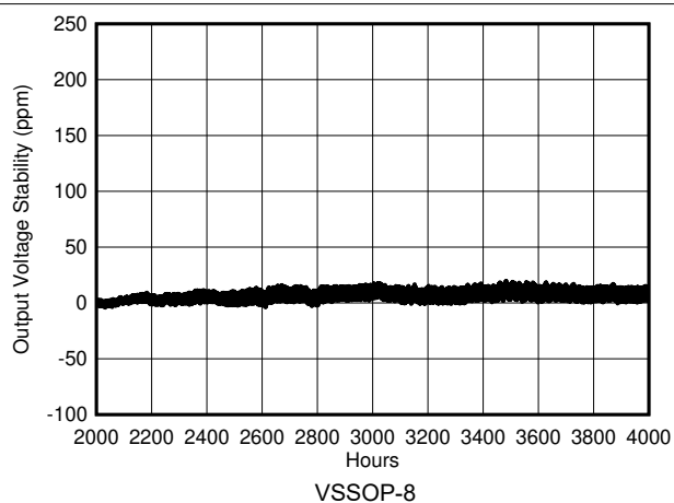
Figure 7-26. REF50xx Long-Term Stability (Second 2000 Hours)
