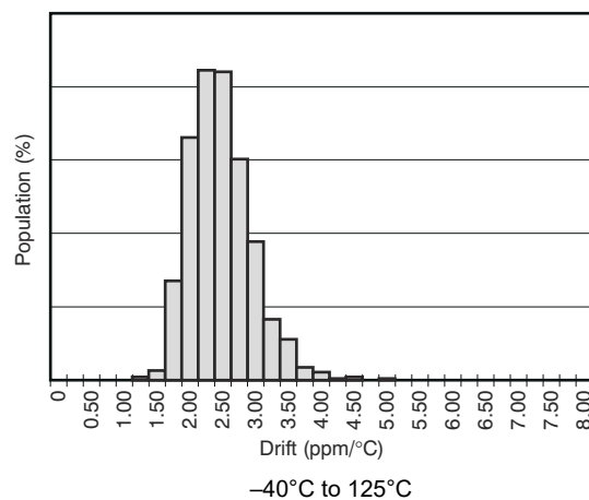
Figure 7-2. Temperature Drift
