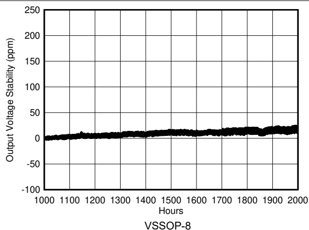
Figure 7-24. REF50xx Long-Term Stability (Second 1000 Hours)
