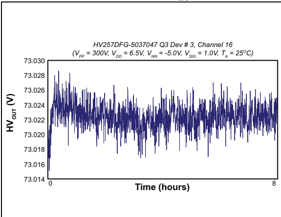
FIGURE 2-12: HV_{OUT} Drift.
