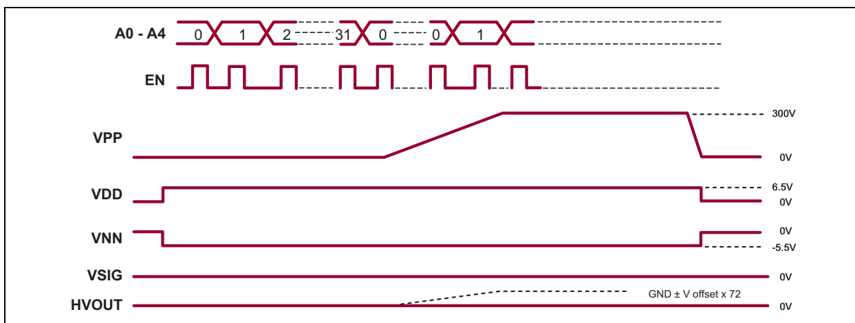
FIGURE 4-2: Recommended Power-up/Power-down Timing.
