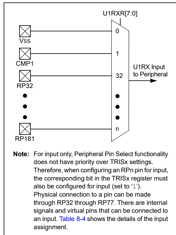
FIGURE 8-2: REMAPPABLE INPUT FOR U1RX
