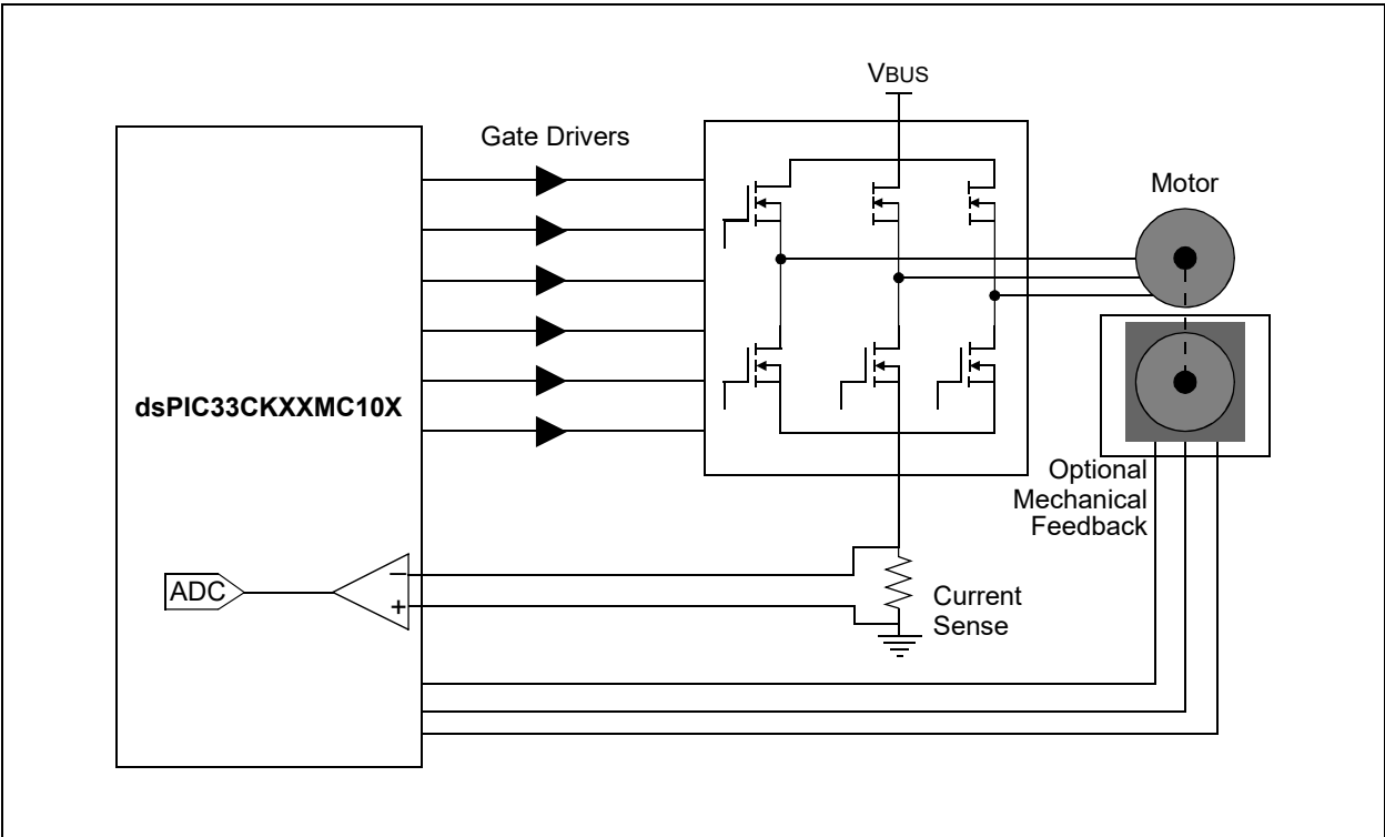
FIGURE 2-6: BLDC MOTOR
