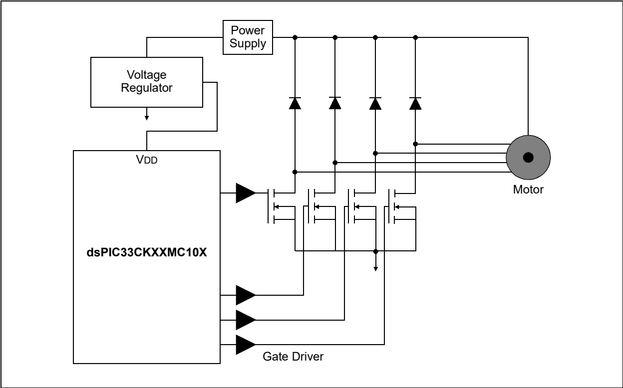
FIGURE 2-5: STEPPER MOTOR
