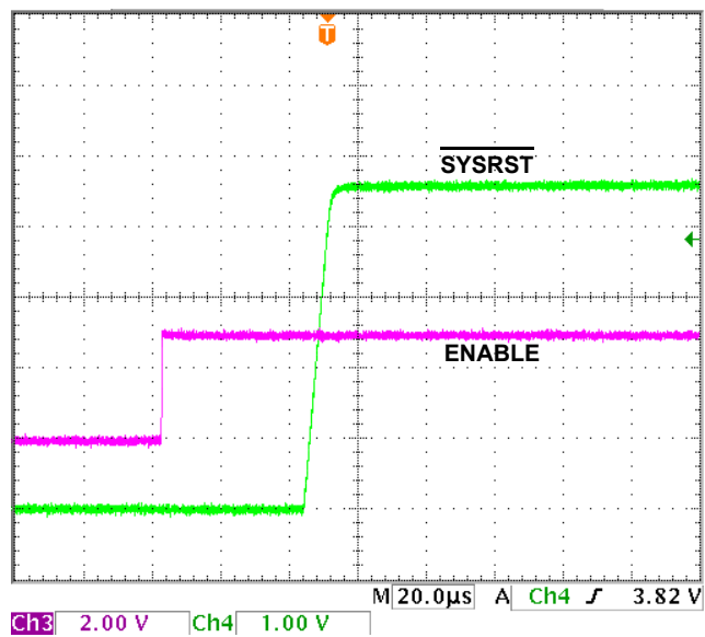
FIGURE 19. 4 UVLOs VALID, ENABLE HIGH TO SYSRST HIGH
