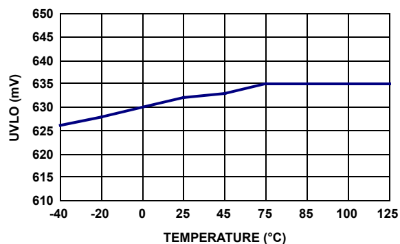
FIGURE 6. UVLO THRESHOLD VOLTAGE
