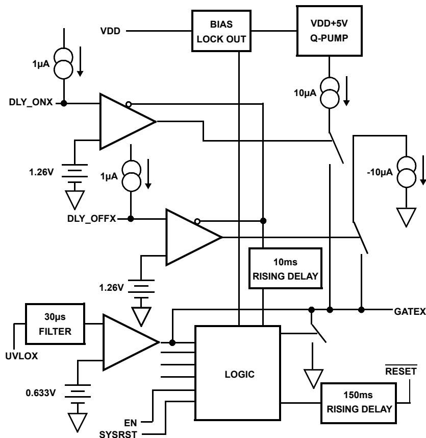
FIGURE 2. ISL8723 BLOCK DIAGRAM (1/4)
