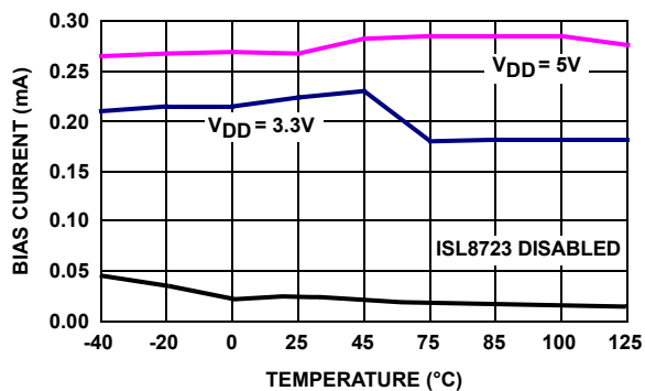
FIGURE 5. BIAS CURRENT
