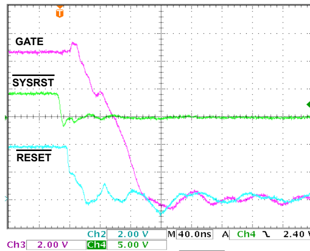
FIGURE 18. SYSRST LOW TO GATE AND RESET LOW
