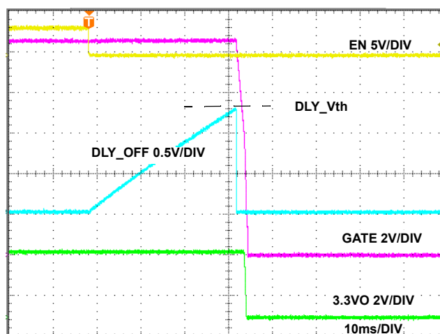
FIGURE 16. ISL8723 3.3V TURN-OFF
