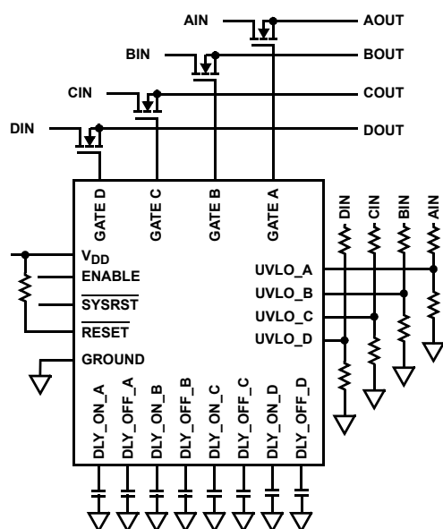
FIGURE 1. TYPICAL ISL8723 APPLICATION USAGE
