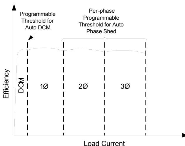
Figure 37: Dynamic Phase Control Regions
