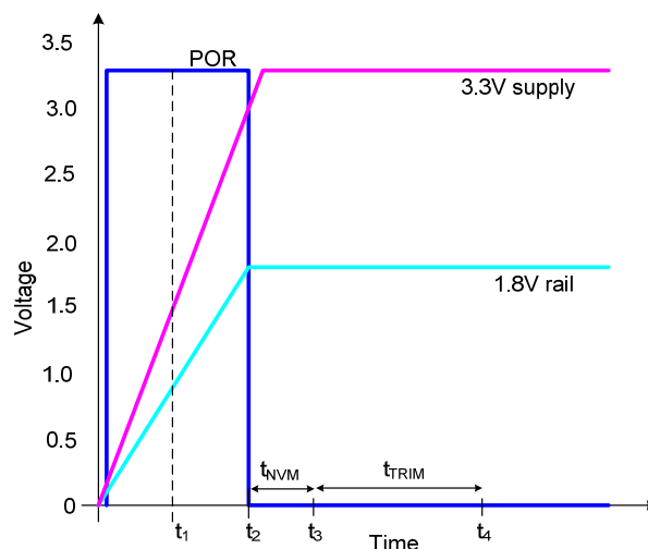
Figure 6: Controller Startup and Initialization
