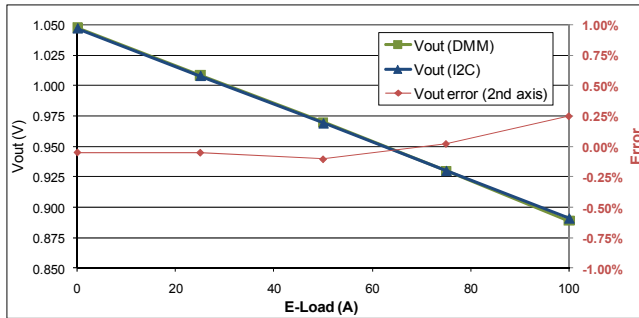
Figure 49: I2C Output Voltage Measurements
