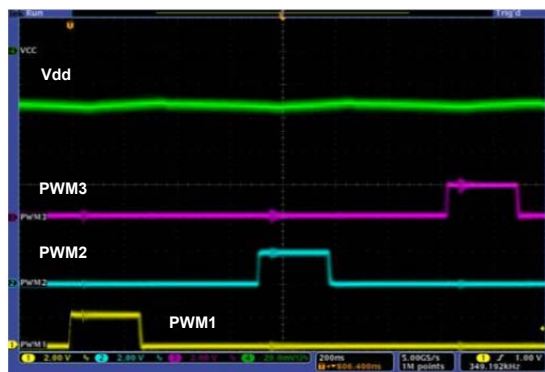
Figure 4: Persistence plot of a 3Φ, 50A system
