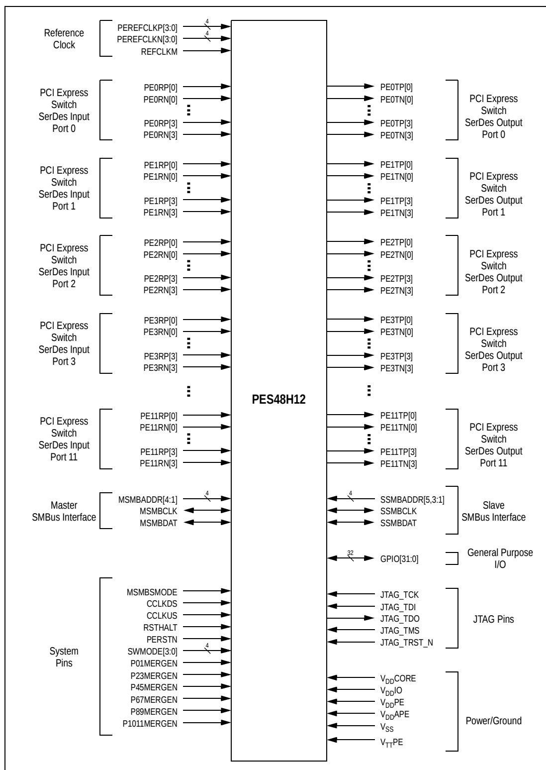
Figure 4 PES48H12 Logic Diagram
