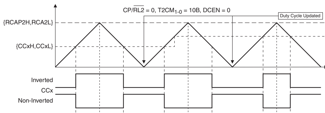
Figure 13-10. Phase and Frequency Correct Symmetrical (Center-Aligned) PWM
