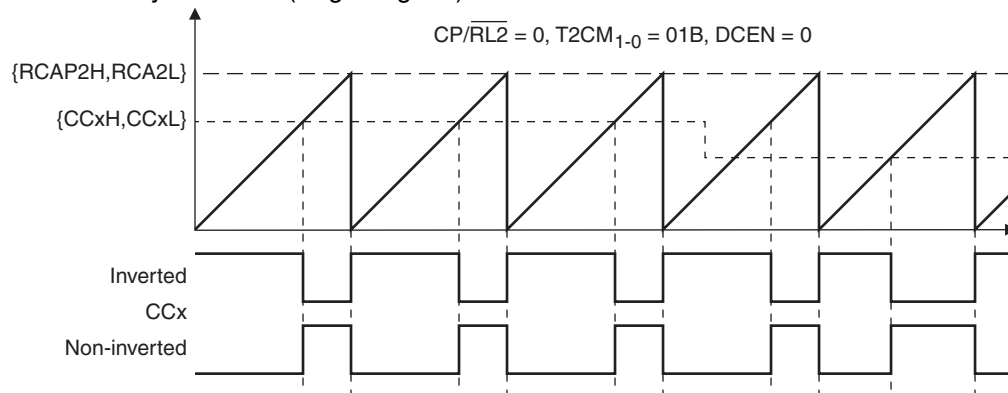
Figure 13-8. Asymmetrical (Edge-Aligned) PWM
