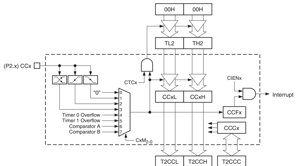
Figure 13-2. CCA Capture Mode Diagram
