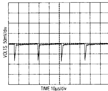
REGULATOR 7 OUTPUT RIPPLE UNFILTERED
