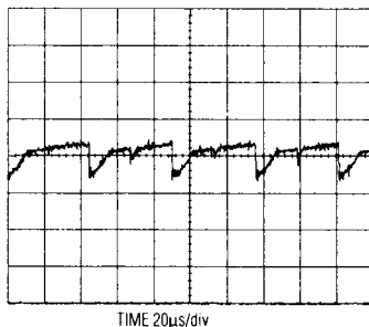
REGULATOR 6 OUTPUT RIPPLE UNFILTERED
