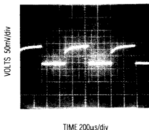
V4 LOAD-TRANSIENT/DROPOUT RESPONSE
