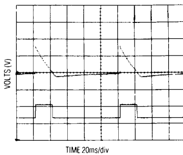
V2 LINE TRANSIENT RESPONSE
