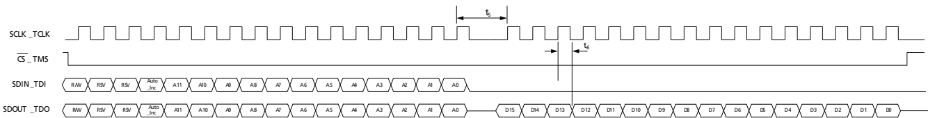
Figure 4-41: Read Mode
