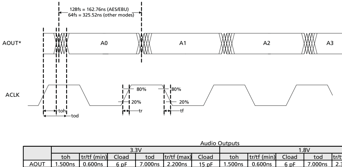
Figure 4-25: ACLK to Data Signal Output Timing
