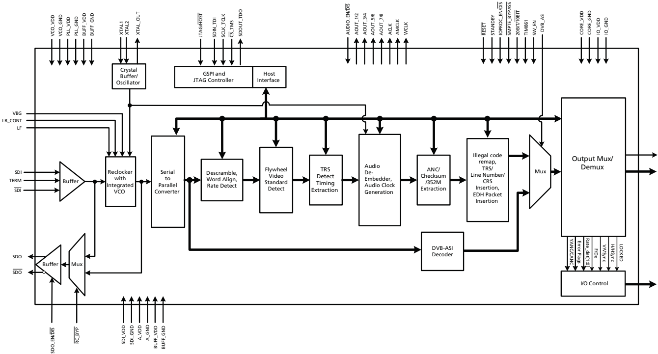
GS1670 Functional Block Diagram
