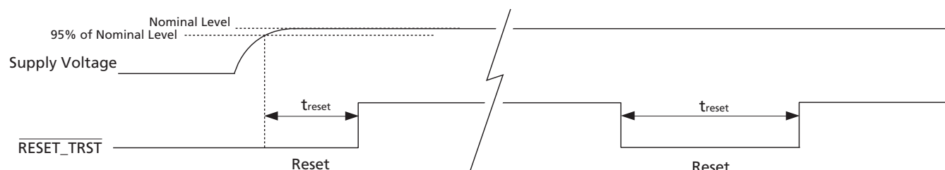
Figure 4-45: Reset Pulse
