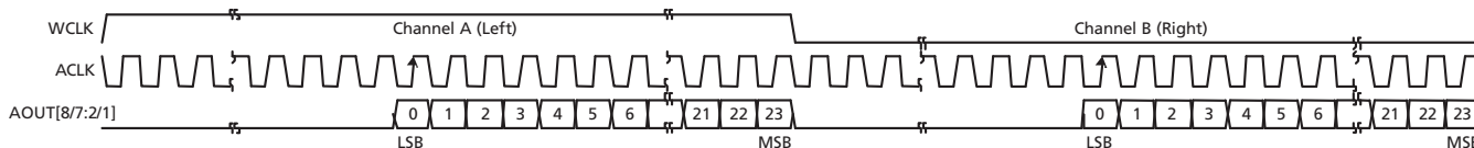
Figure 4-31: Serial Audio, Right Justified, LSB First
