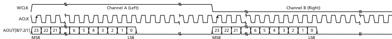
Figure 4-28: Serial Audio, Left Justified, MSB First
