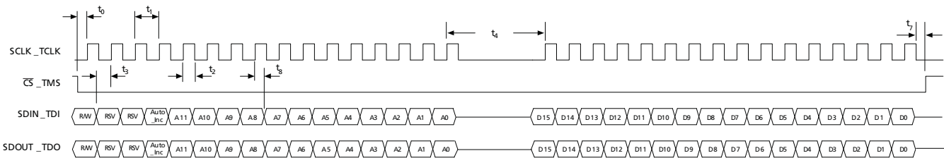
Figure 4-40: Write Mode
