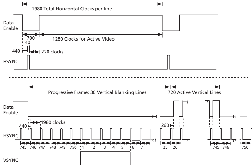
Figure 4-14: H:V:DE Output Timing 1280 x 720p @ 50 (Format 19)
