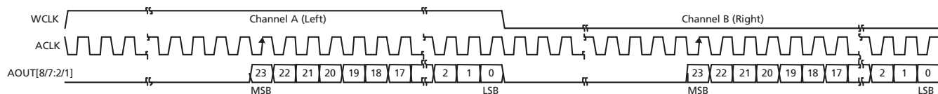
Figure 4-30: Serial Audio, Right Justified, MSB First
