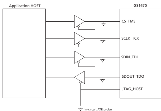
Figure 4-43: In-Circuit JTAG
