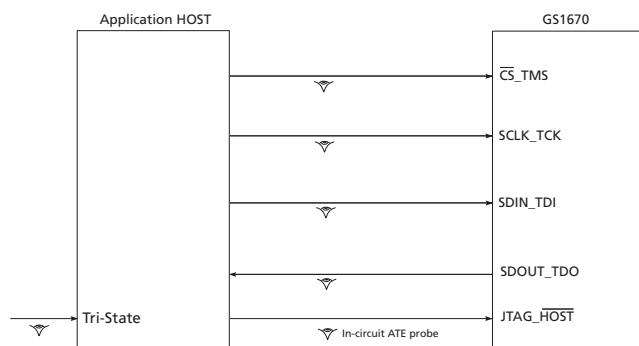
Figure 4-44: System JTAG
