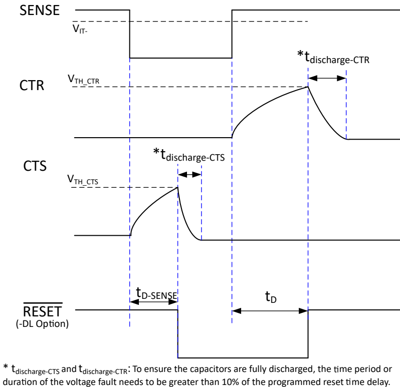
Figure 8-2. CTS and CTR Charge and Discharge Behavior Relative to SENSE and \overline{RESET}
