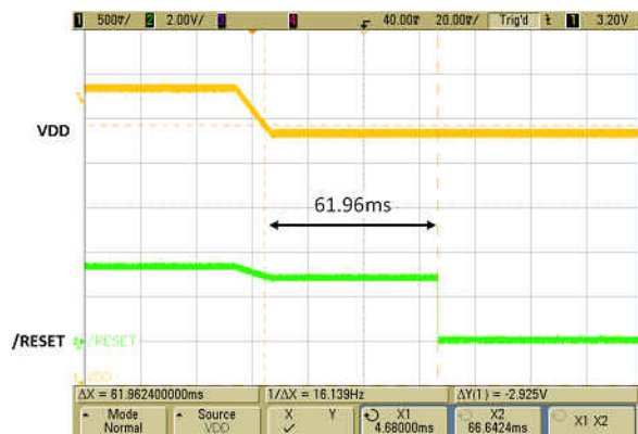
Figure 9-3. Sense Delay
