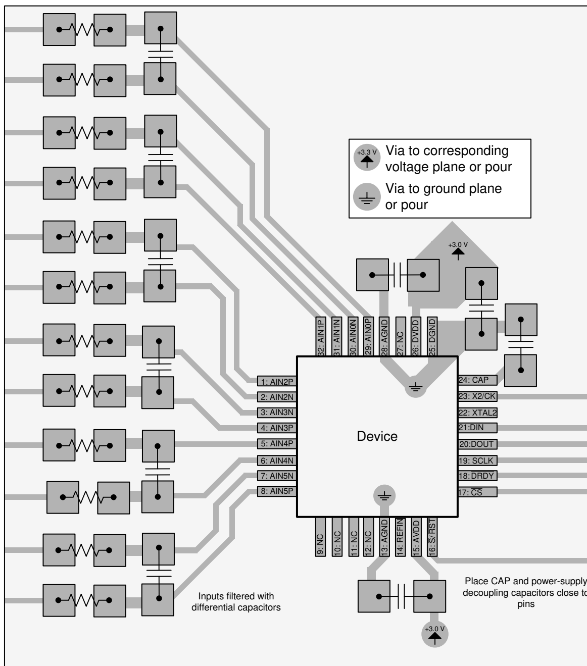
Figure 9-6. Layout Example
