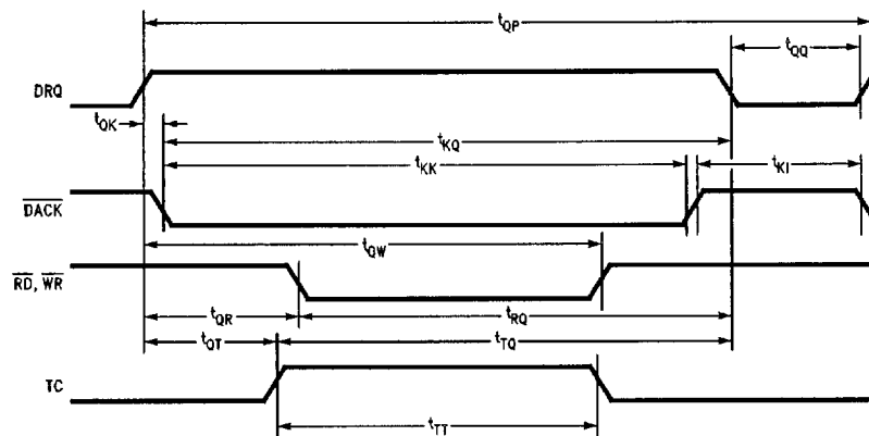
FIGURE 9-8. DMA Timing
