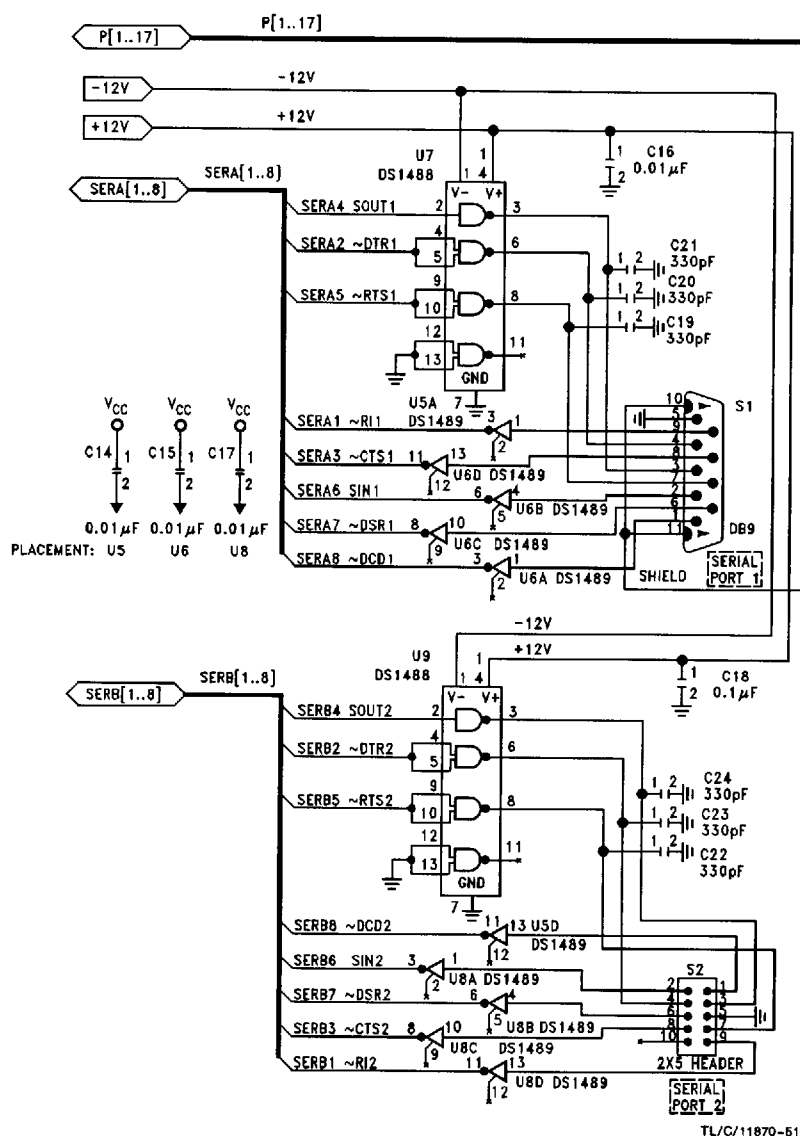
FIGURE 10-3. PC87322VF Adapter Card Schematic (Continued)
