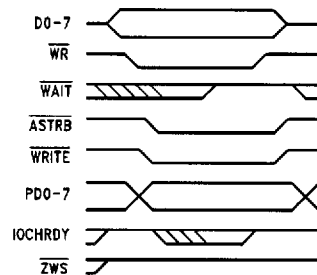
FIGURE 7-1. EPP 1.7 Address Write
