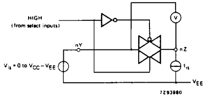
Fig. 8 Test circuit for measuring R_{ON} .
