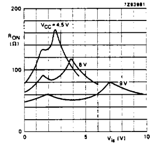
Fig. 9 Typical R_{ON} as a function of input voltage V_{1s} for V_{1s} = 0 to V_{CC} - V_{EE} .
