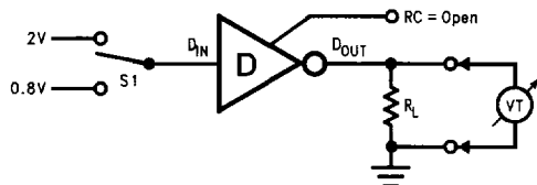
FIGURE 1. Driver DC Test Circuit
